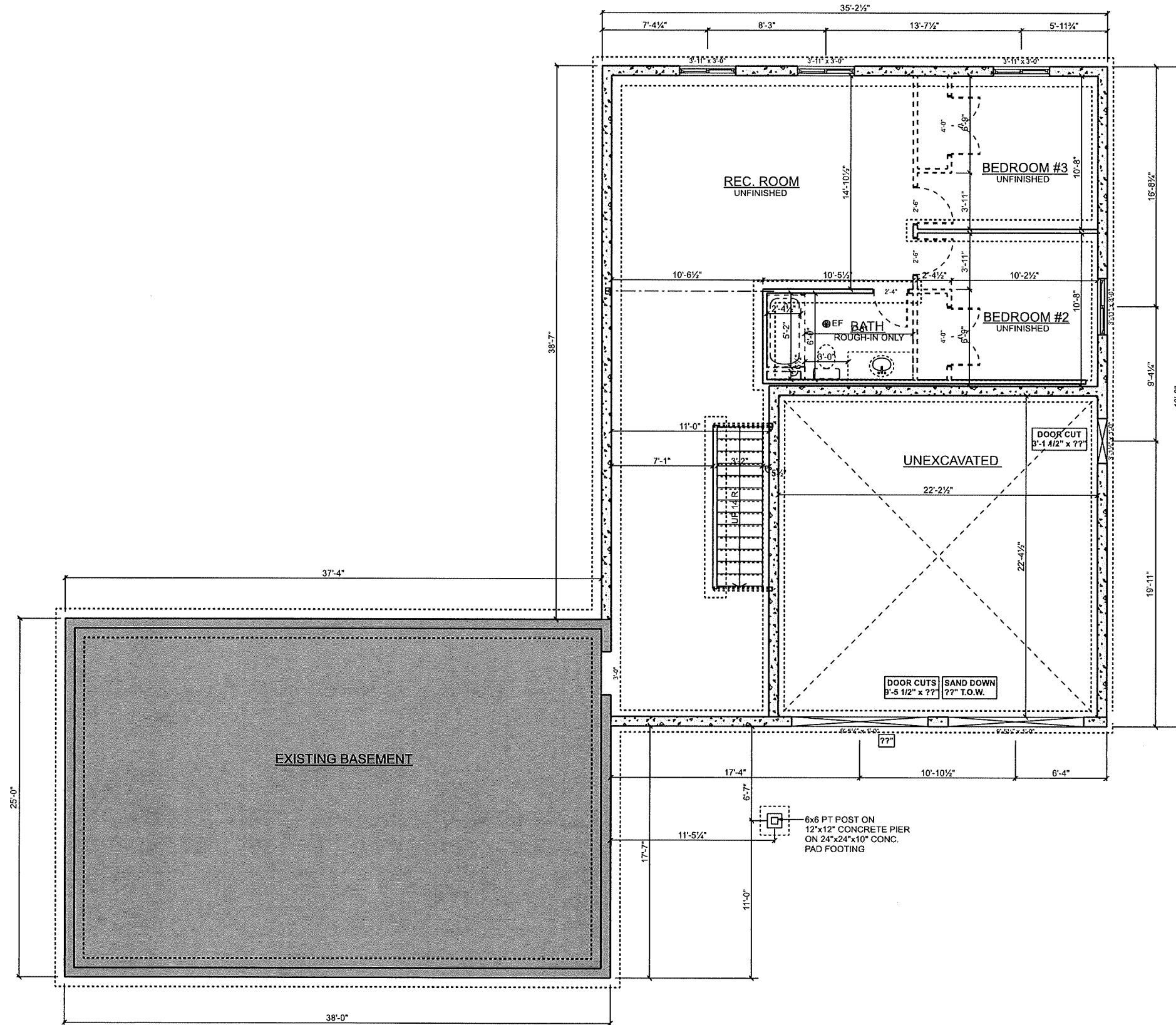
BASEMENT PLAN SCALE: 1/8" = 1'-0"
